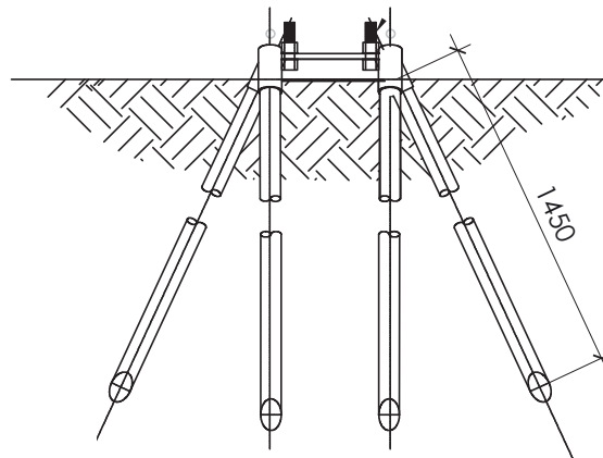
TYPICAL SECTION- S250 NTS
