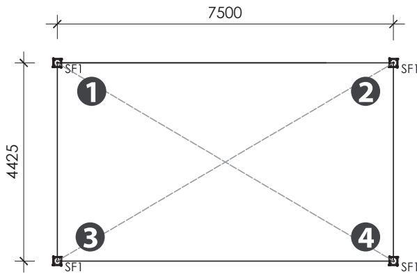
SUREFOOT PLAN LAYOUT NTS
